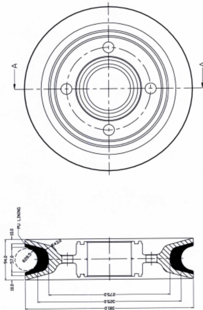
① PULLEY
