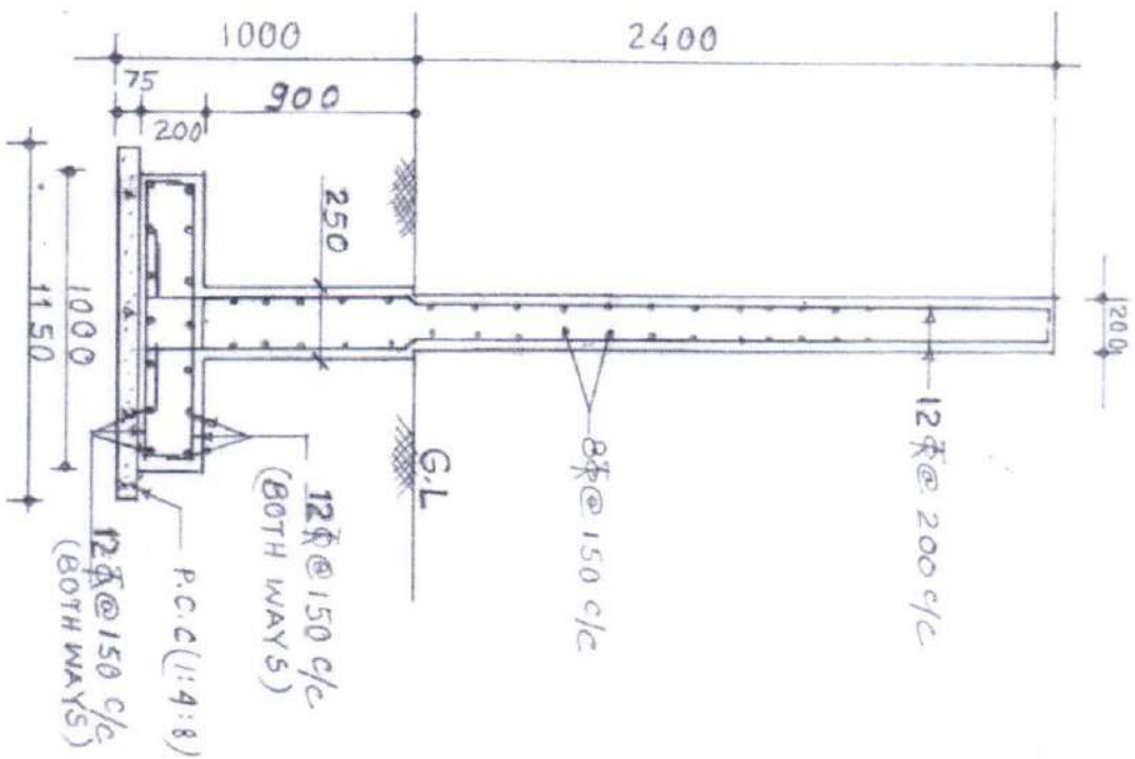
R/F DET OF R.C.C. BOUNDARY WALL
