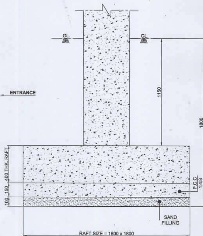
FOUNDATION SECTION (SCALE - 1 : 12)
