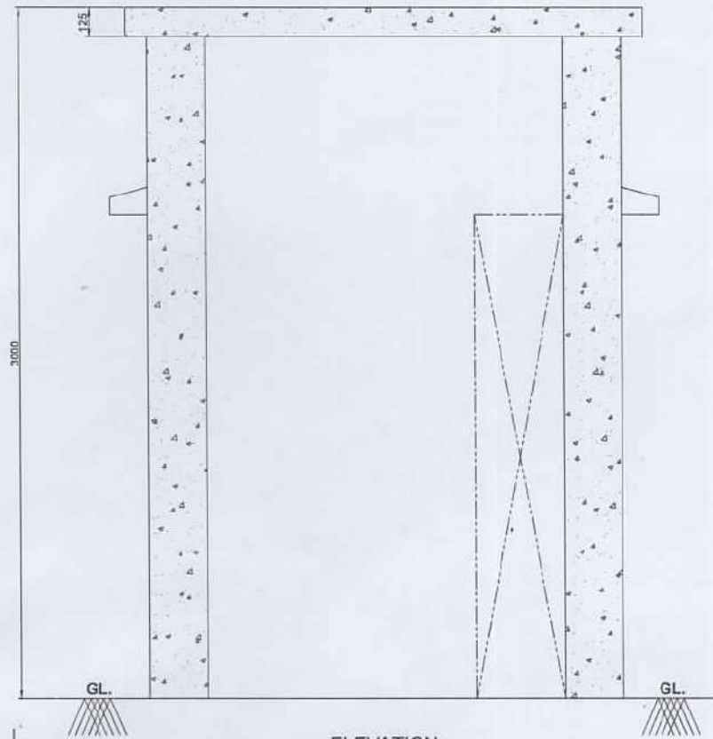
ELEVATION (SCALE - 1 : 12)
