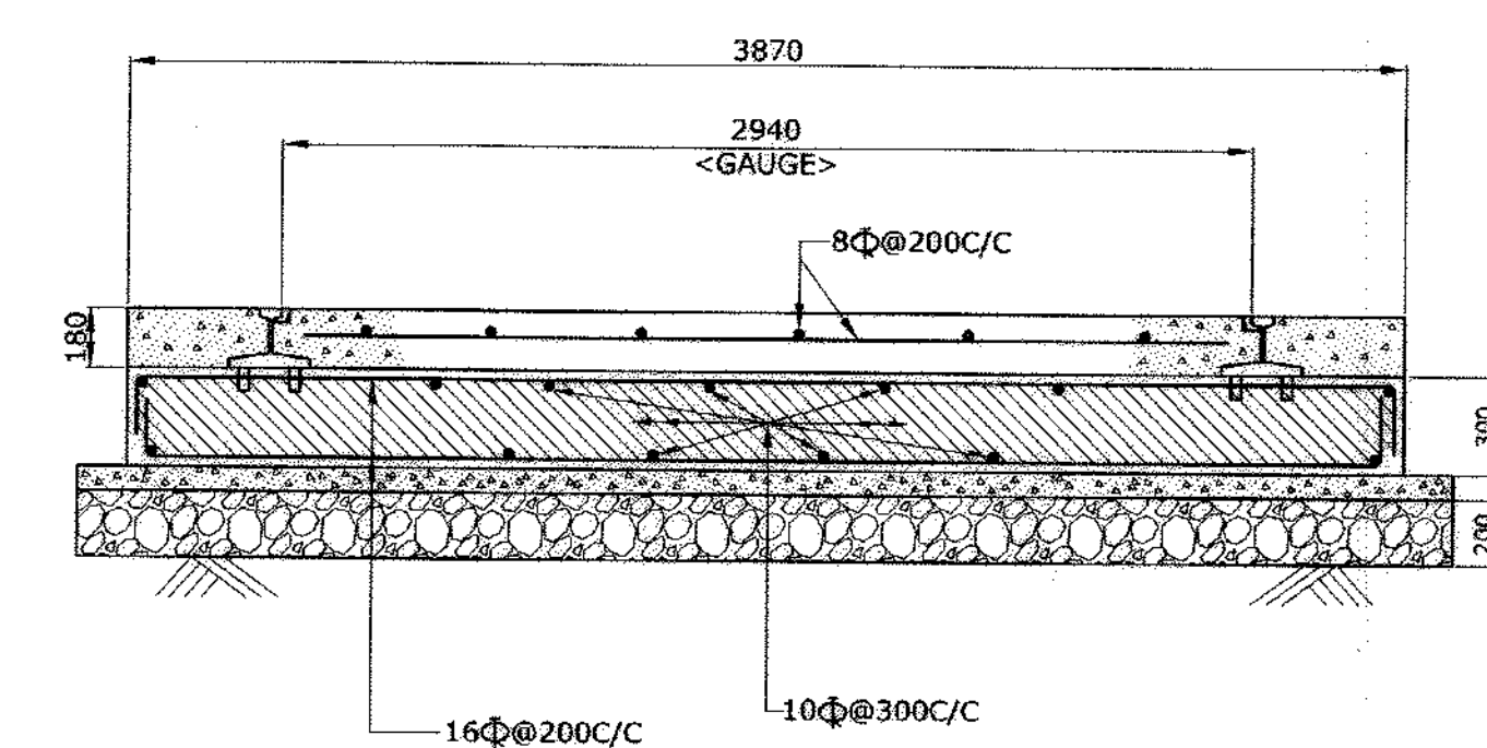
SECTION 2-2
