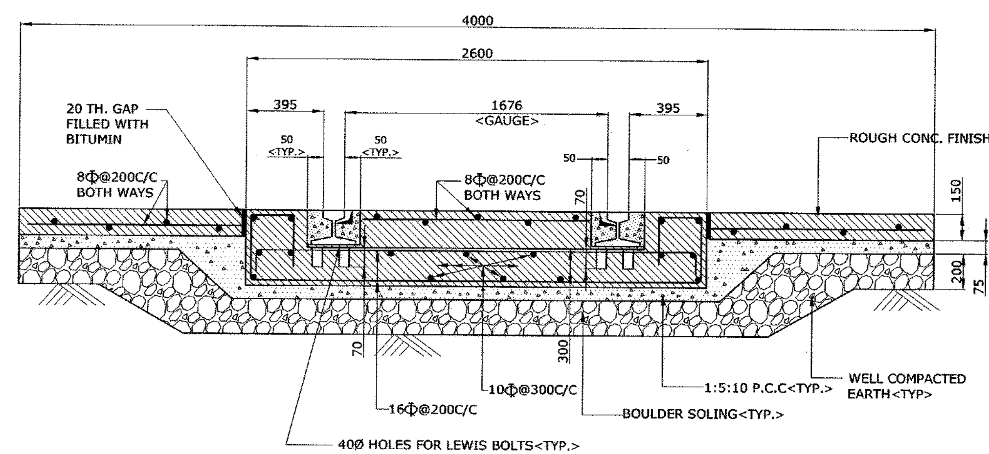
SECTION 1-1
