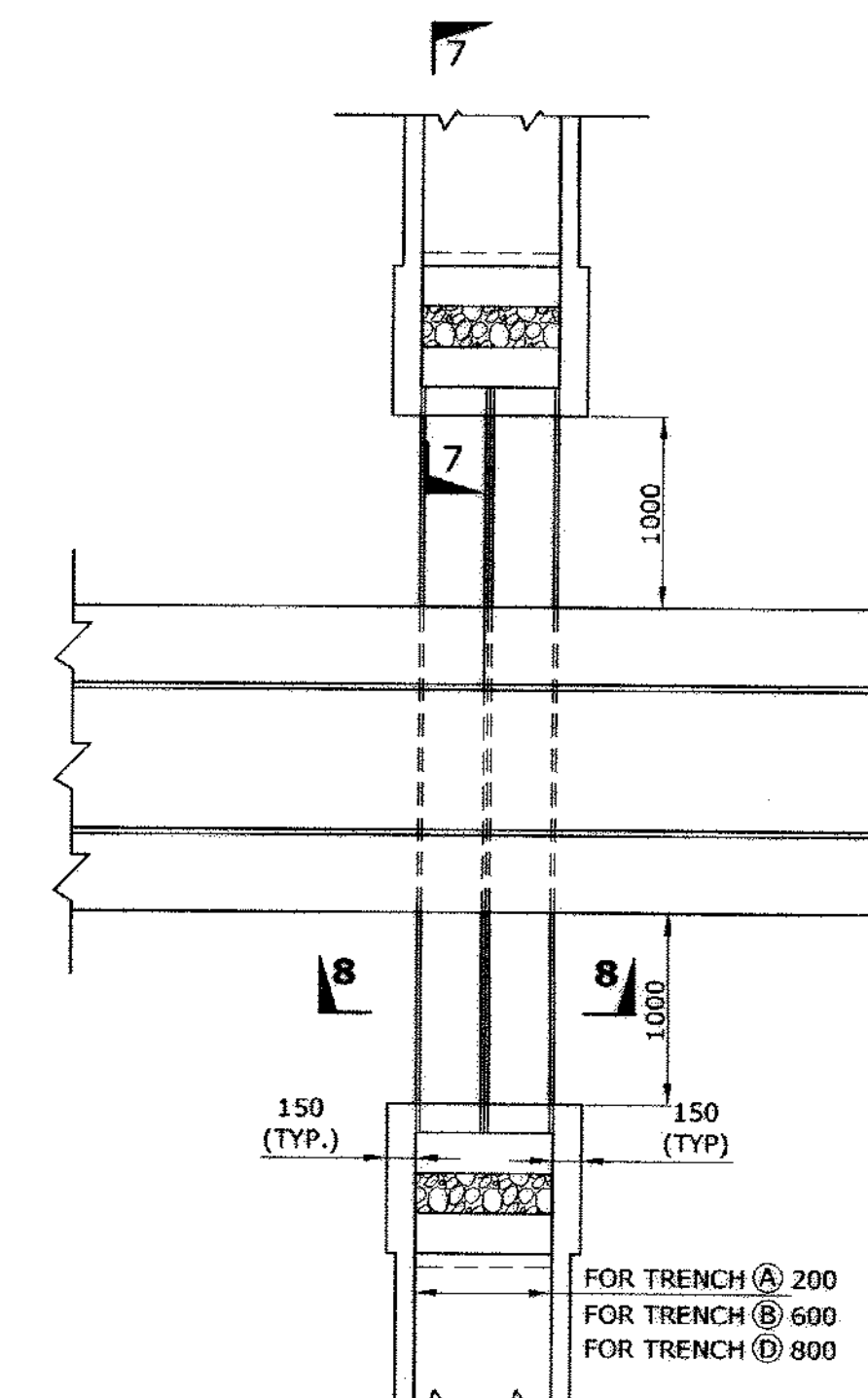
TYPICAL CABLE TRENCH & RAIL-CUM-ROAD CROSSING
