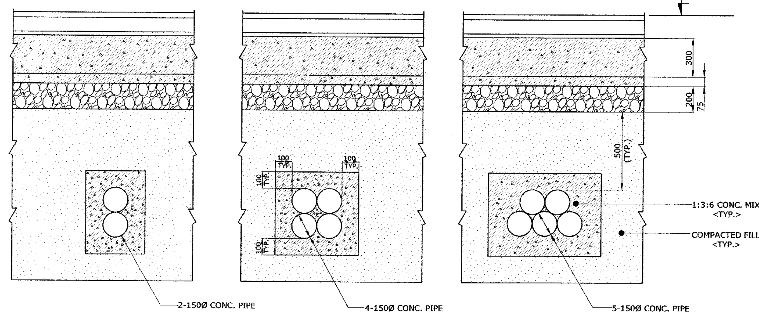
TRENCH TYPE - (A)
