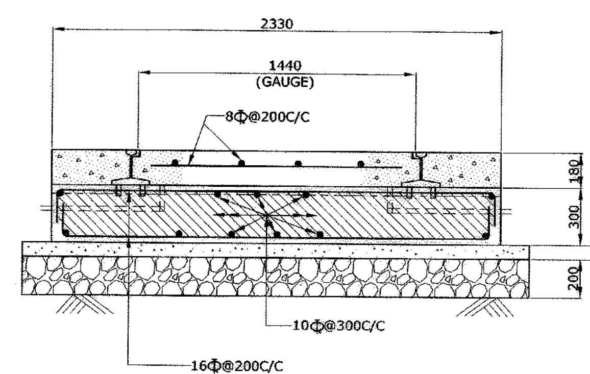
SECTION 4-4
