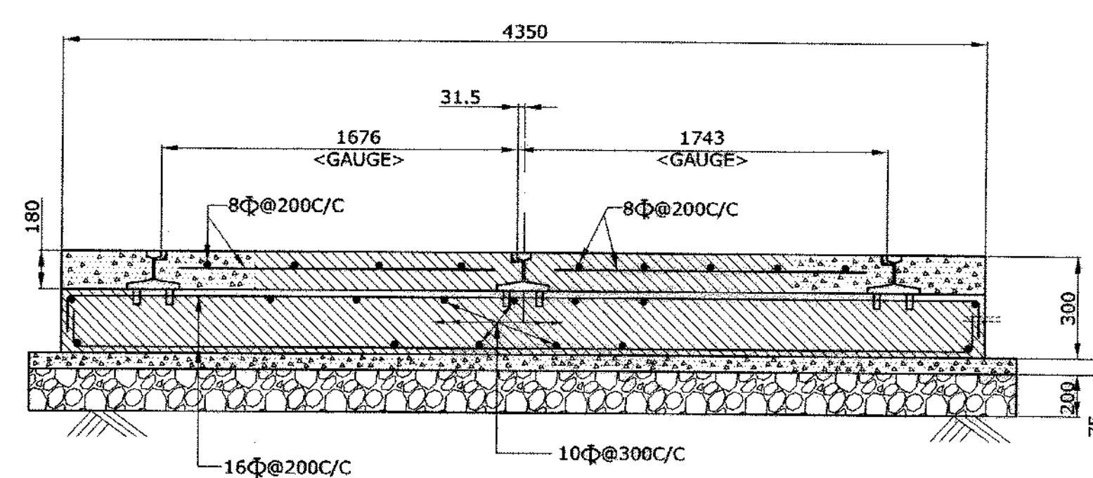
SECTION 3-3
