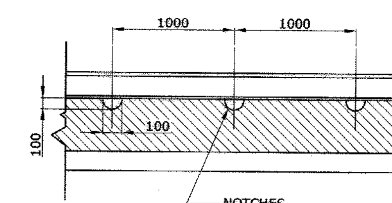
SECTION 10-10 <TYP DETAIL OF NOTCHES>
