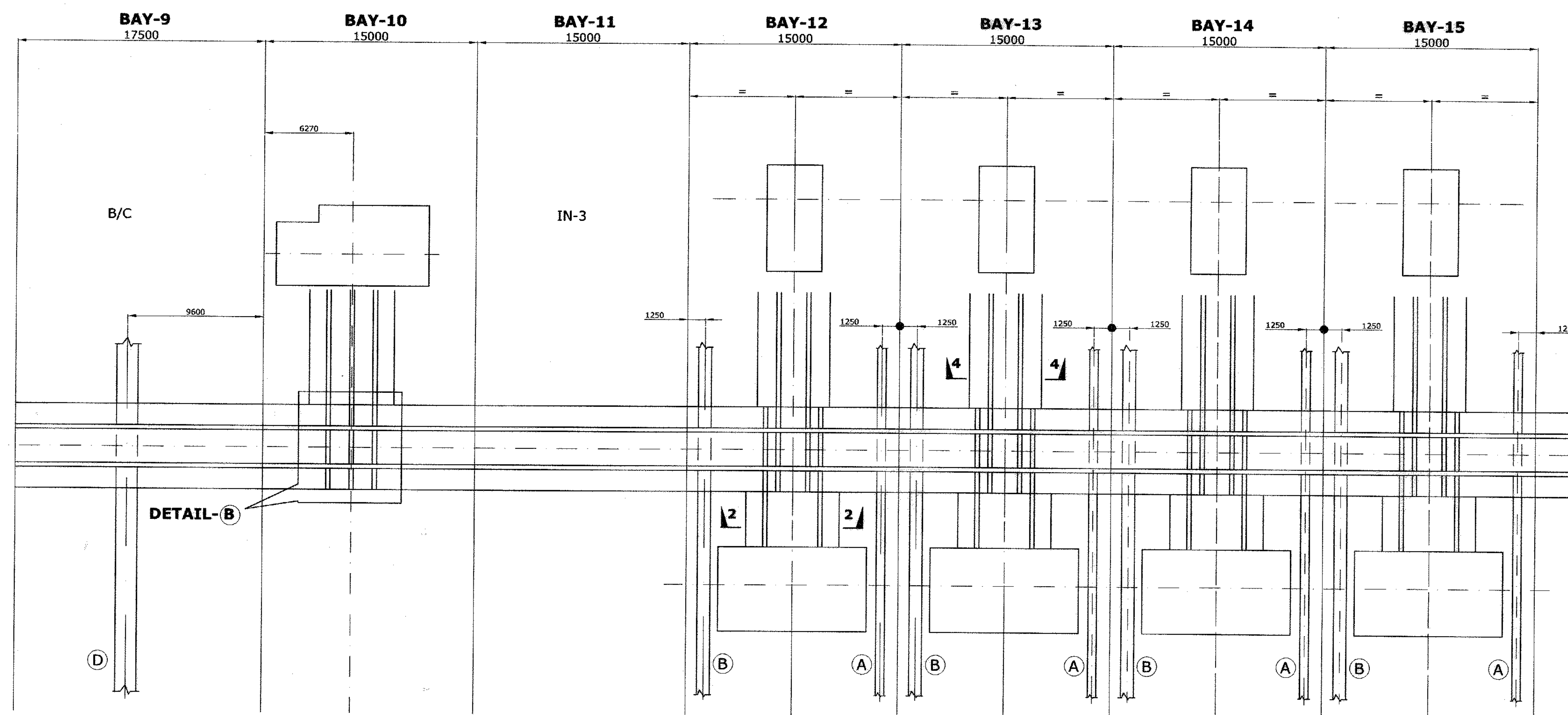
LAYOUT OF RAIL CUM ROAD & RAIL TRACK
